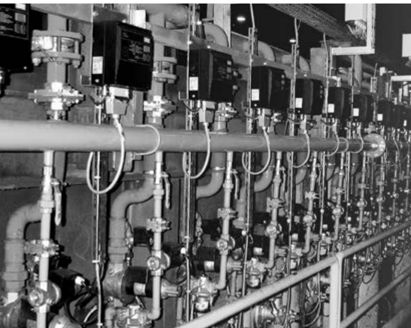
Hardening furnace with lots of industrial burners located side-by-side
