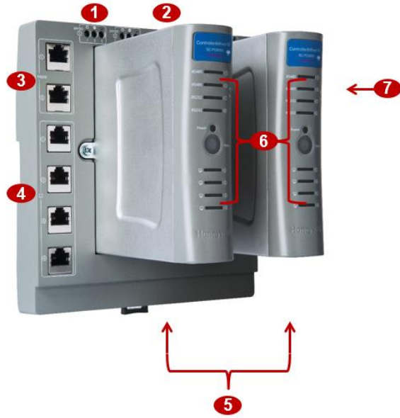
Figure 3 –Redundant Controller Hardware Summary
