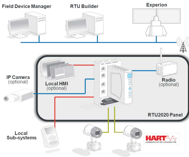
Figure 1 – Sample RTU System Architecture
