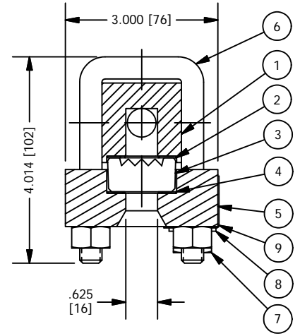
SECTION X-X SERIES R-20
