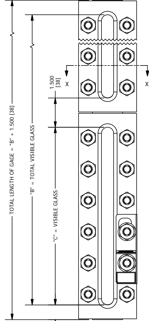
FRONT VIEW REFLEX & TRANSPARENT SERIES 20 GAGES
