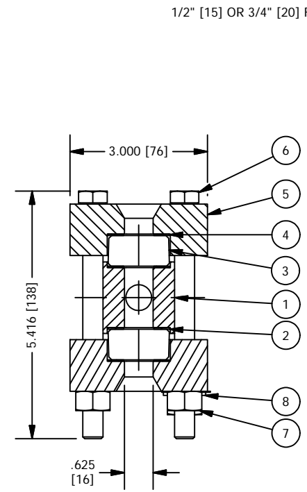
SECTION X-X SERIES T-20
